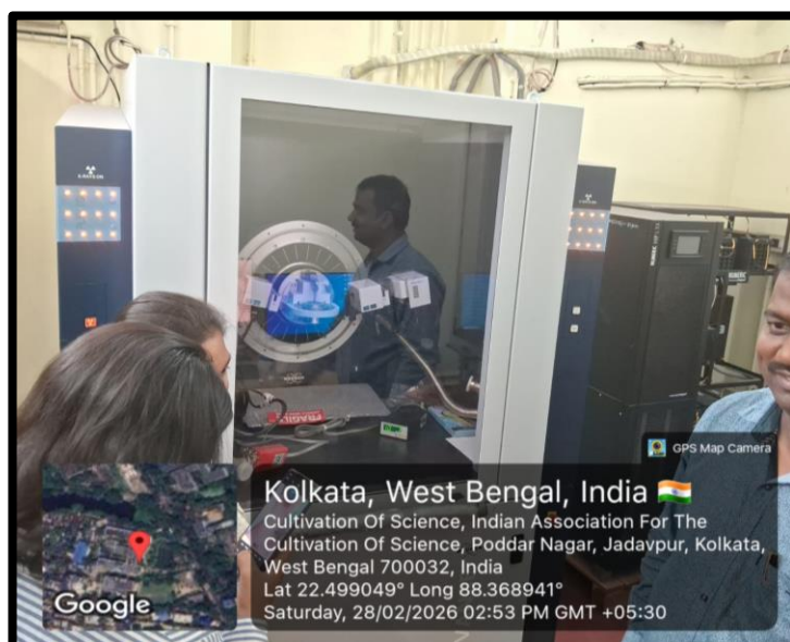
Powder XRD
